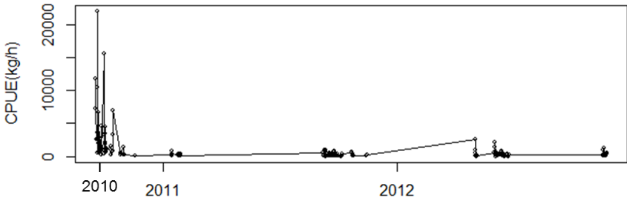
Figure 12: Time-series of catch per unit of effort (CPUE, kg/trawl hour), i.e. set-by-set data, for pelagic armourhead from 2010 to 2013. Source: observer reports submitted to SEAFO.
